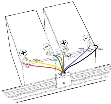
Dual mSensor
