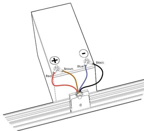
Single mSensor
