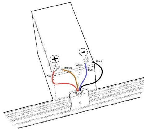
Single mSensor
